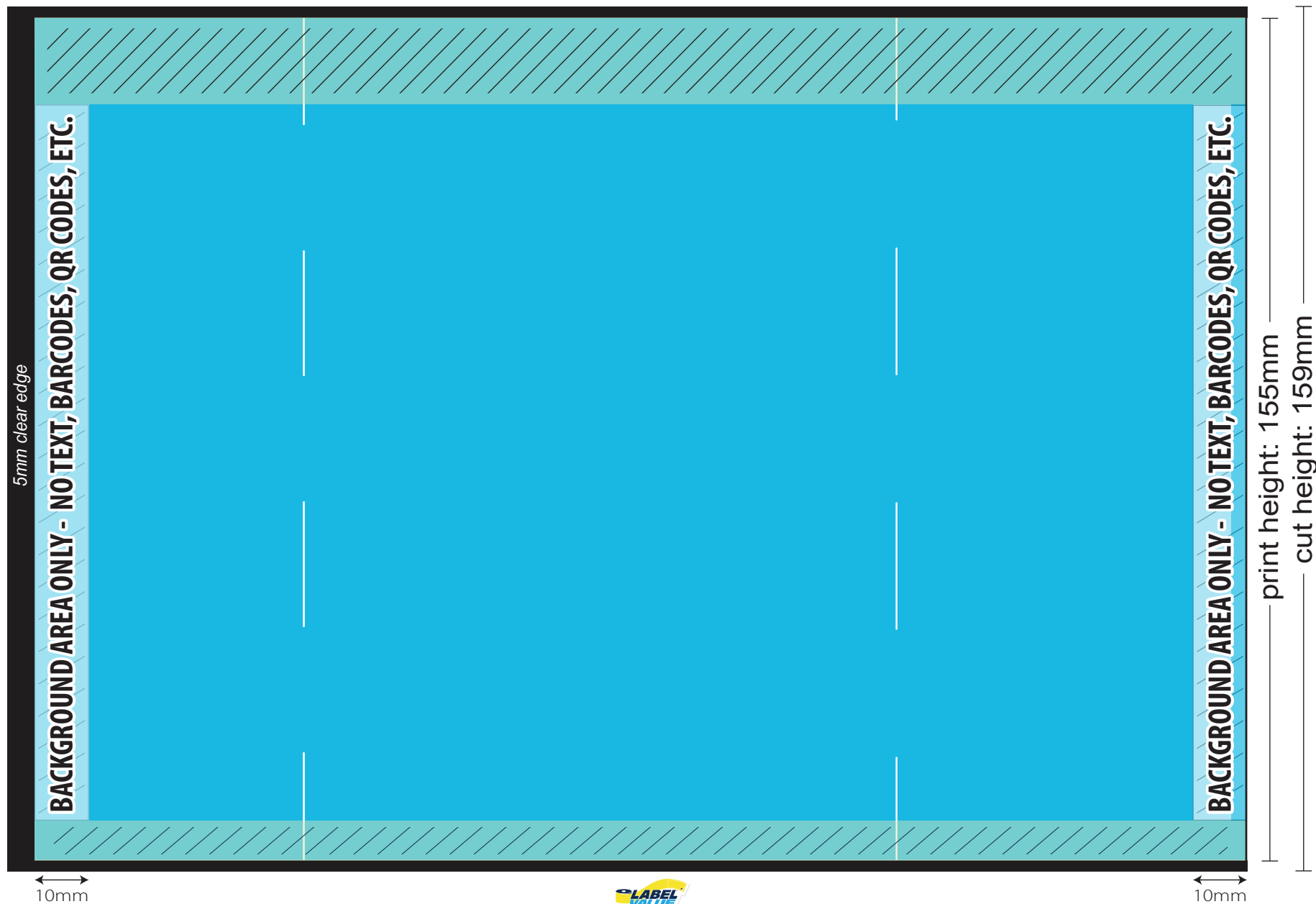
16 OZ STANDARD SHRINK SLEEVE TEMPLATE
