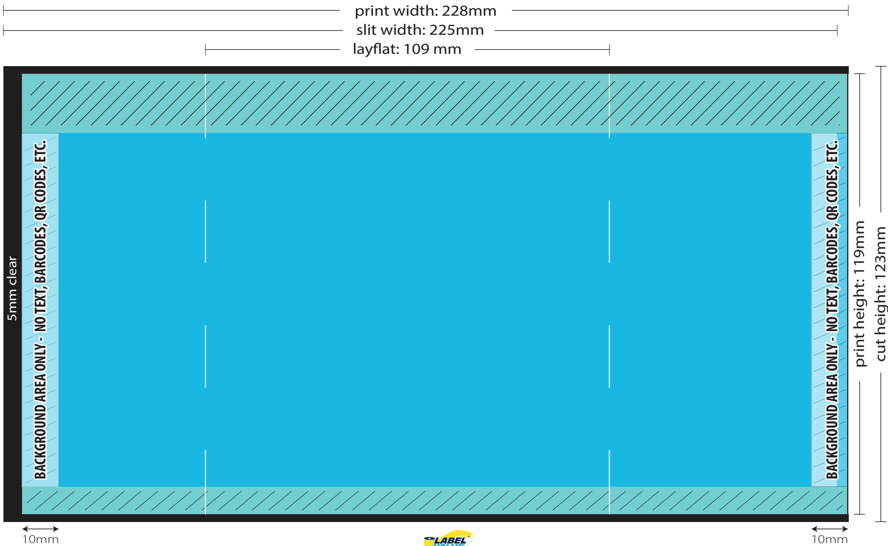
12 OZ STANDARD SHRINK SLEEVE TEMPLATE
